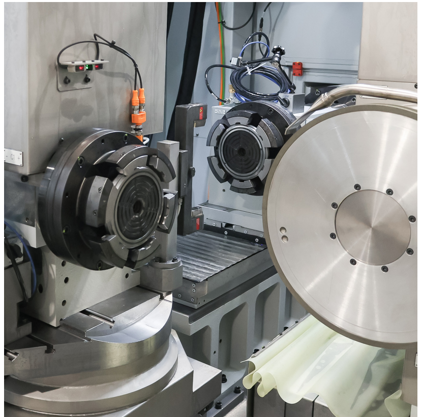
KELLENBERGER U300 BoulePro for SiC transformation from boule to puck
