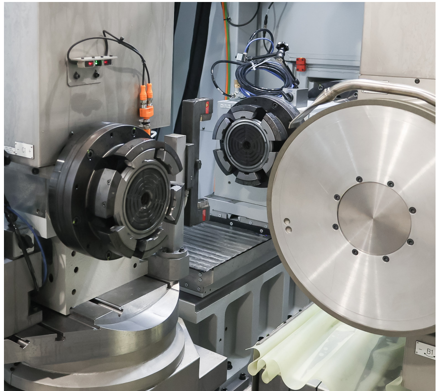
USACH Boule Pro 200AX for SiC transformation from boule to puck
